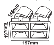
Dimension ( mm )
